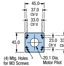
Reverse SM 16
