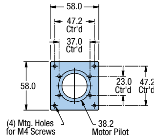
Reverse NEMA 23
