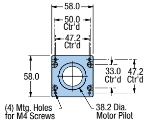
In-line NEMA 23
